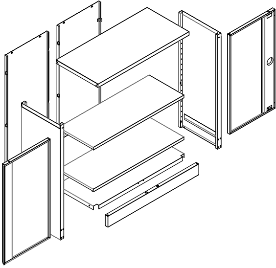
NON-ASSEMBLED VIEW
